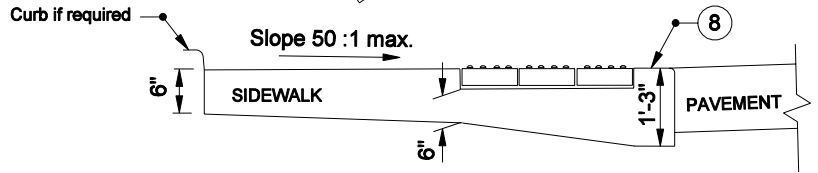
SECTION C-C
