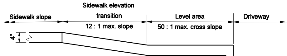
SECTION B - B SIDEWALK ELEVATION TRANSITION
