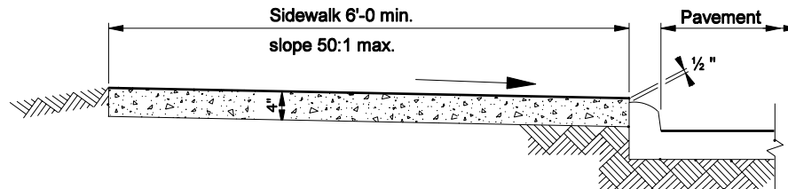
SECTION A - A SIDEWALK ADJACENT TO CURB
