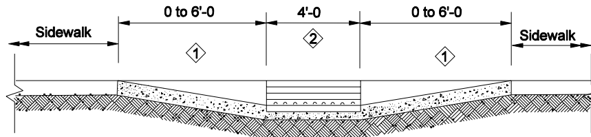
SECTION B-B
