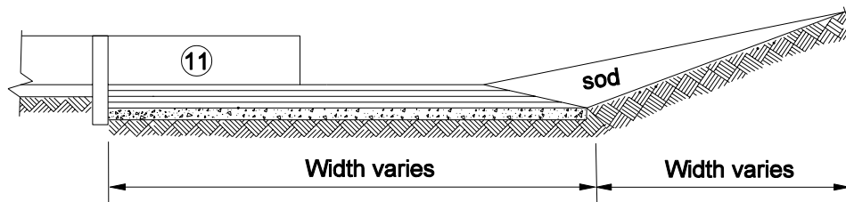
SECTION B-B
